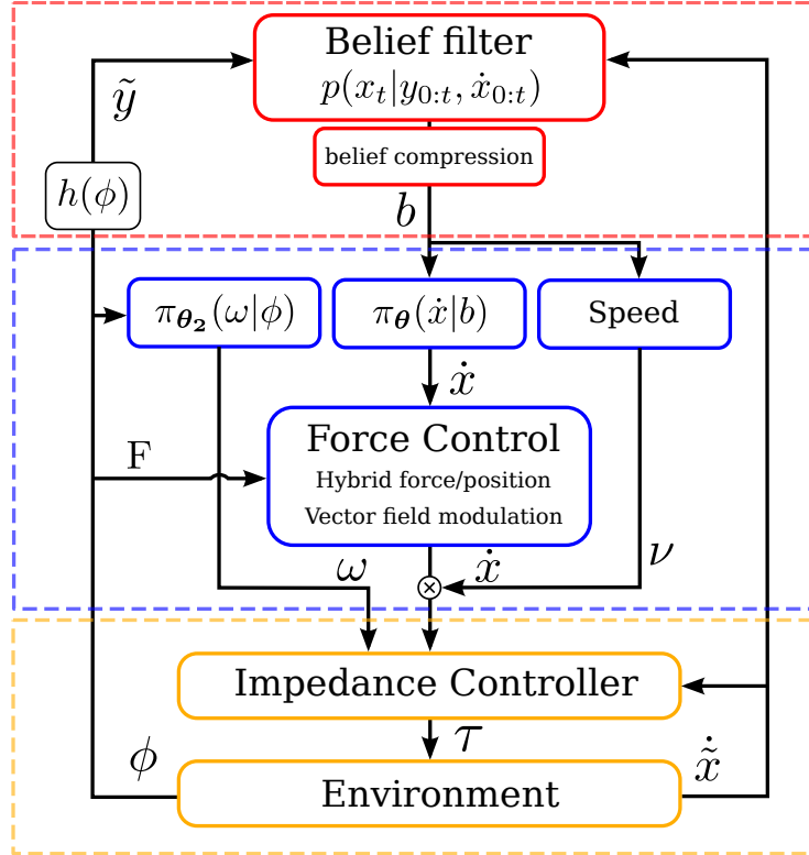
Figure 4.12: Control architecture. The PMF (belief) receives a measured velocity, \dot{x} , and a sensor measurement \tilde{y} and is updated via Bayes rule. The belief is compressed and used by both the GMM policy and the proportional speed controller, Equation 4.5.5.
