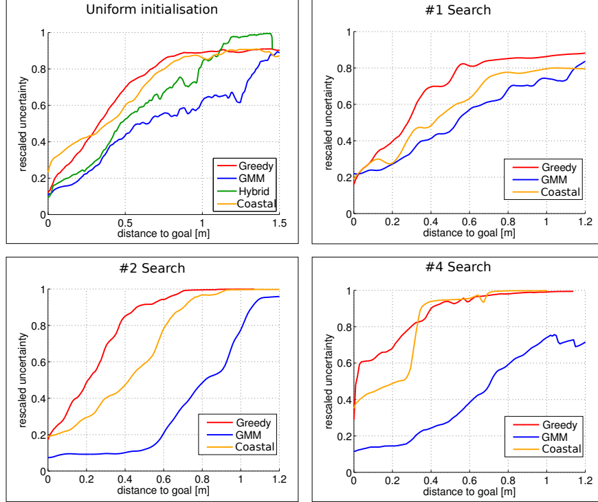
Figure 3.14: Reduction of the uncertainty for the Uniform, #1, #2 and #4 experiment, the expected value is reported Top left : Uniform initialisation, expected uncertainty for the Greedy (red), GMM (blue), Hybrid (green) & Coastal (orange) search strategies. Top right : Experiment #1. Bottom left : Experiment #2. Bottom right : Experiment #4.
