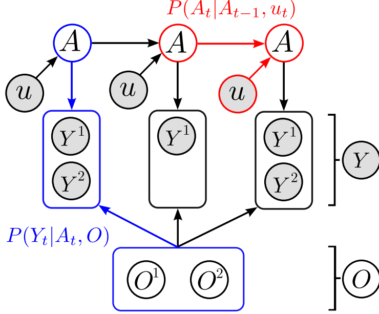
Figure 5.3: Directed graphical model of dependencies between the agent(A) and object(O)'s estimated location. Each object, O^{(i)} is associated with one sensing random variable Y^{(i)} . The overall sensing random variable is Y = [Y^{(1)}, \dots, Y^{(M-1)}]^T , where M is the total number of agent and object random variables in the filter. For readability we have left out the time index t from A and Y . Since the objects are static, they have no temporal process associated with them thus they will never have a time subscript. The two models necessary for filtering are the motion model P(A_t|A_{t-1}, u_t) (red) and measurement model P(Y_t|A_t, O) (blue).
