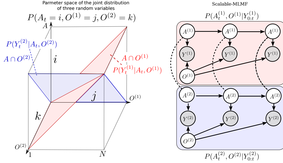
Figure 5.12: Left: Joint distribution P(A, O^{(1)}, O^{(2)}) of the agent and two objects. Each measurement likelihood function, P(Y|A, O^{(1)}) , P(Y|A, O^{(2)}) corresponds to a hyperplane in the joint distribution. The state space is discretised to N bins giving the total number of parameters in the joint distribution of N^3 . Right: Scalable-MLMF Each agent-object joint distribution pair is modelled independently. For clarity we have left out the action random variable u which is linked to every agent node. Two joint distributions P(A^{(1)}, O^{(1)}|Y_{0:t}^{(1)}) and P(A^{(2)}, O^{(2)}|Y_{0:t}^{(2)}) parametrise the graphical model. The dashed undirected lines represent a wanted dependency, if present O^{(1)} and O^{(2)} are to be dependent through A . In the standard setting there will be no exchange of information between the individual joint distributions. However we demonstrate later on how we perform a one time transfer of information when one of the objects is sensed.
