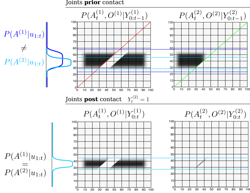
Figure 5.13: Transfer of information (joint distributions) Top: Joint distributions of P(A_t^{(1)}, O^{(1)}|Y^{(1)}) and P(A_t^{(2)}, O^{(2)}|Y^{(2)}) prior sensing, Y_t^{(2)} = 1 , see Figure 5.14 ( Top right ) for the corresponding marginals. The red and green lines across the joint distributions correspond to the region in which the likelihood functions P(Y_t^{(1)}|A_t^{(1)}, O^{(1)}) and P(Y_t^{(2)}|A_t^{(2)}, O^{(2)}) will change the joint distributions. The dotted blue lines are to ease the comparison of the joint distributions prior and post sensing. Bottom right: After the agent has sensed O^{(2)} , all the probability mass which was not overlapping the green line becomes an infeasible solution to the agent and object locations. At this point the marginals P(A_t^{(1)}|u_{1:t}) \neq P(A_t^{(2)}|u_{1:t}) are no longer equal (see the blue marginals Top ). Bottom left: The constraint imposed by the likelihood function of the second object (green line) is transferred to the joint distribution of the first object according to Algorithm 4. This results in a change in the joint distribution P(A_t^{(1)}, O^{(1)}|Y^{(1)}) , which satisfies the constraints imposed by the agent's marginal from the joint distribution P(A_t^{(2)}, O^{(2)}|Y^{(2)}) .
