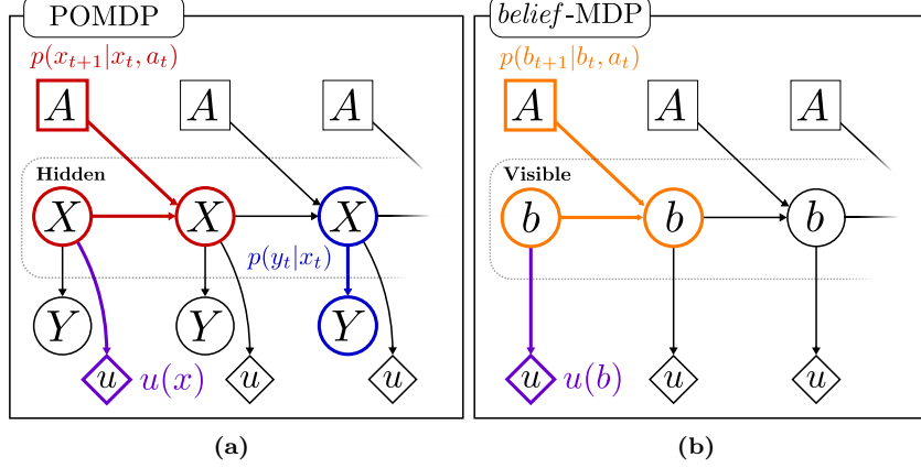
Figure 2.6: (a) POMDP graphical model. The state space, X , is hidden, but is still partially observable through a measurement, Y . (b) The POMDP is cast into a belief Markov Decision Process, belief-MDP. The state space is a probability distribution, b(x_t) = p(x_t) , (known as a belief state) and is no longer considered a latent state. The original state transition function p(x_{t+1}|x_t, a_t) is replaced by a belief state transition, p(b_{t+1}|b_t, a_t) . The reward is now a function of the belief.
