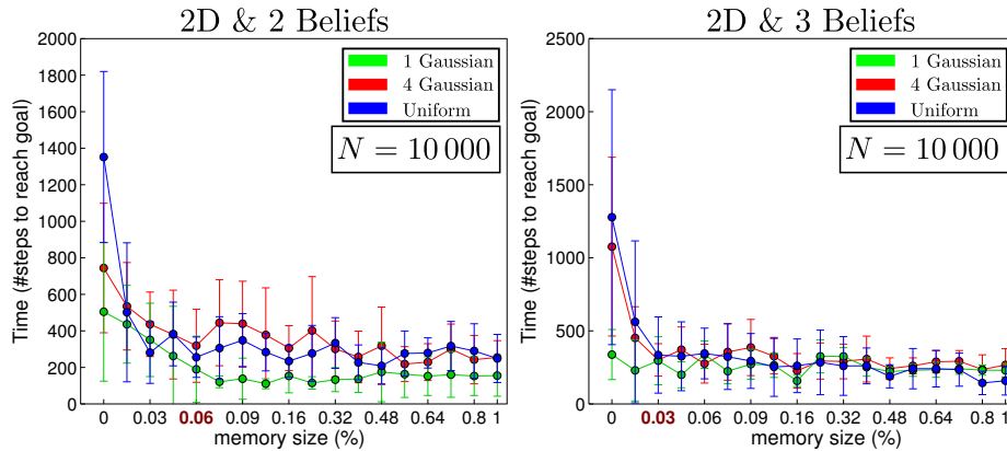
Figure 5.19: Memory size vs time to find objects in 2D. The initial beliefs correspond to those of Figure 5.17, a) for Gaussian (green line), b) 4 Gaussians (red line) and c) Uniform (blue line), both objects are initialised according to d) and e).
