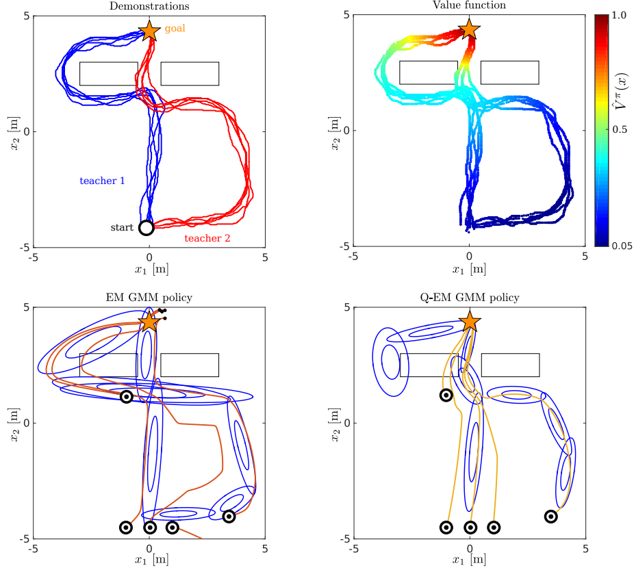
Figure 4.7: Fitted policy evaluation & improvement example. Top-left: The goal of the task is to reach the goal state. The first teacher (blue) demonstrates five trajectories which contours the obstacle in front of the goal. The second teacher (red) demonstrates 5 trajectories which initially deviate from the goal before passing between the two obstacles. Bottom-left: The EM algorithm is used to fit a GMM to the teachers' original data. The marginal \pi_{\theta}(x) is plotted in blue and trajectories generated by the policy \mathbb{E}\{\pi_{\theta}(\dot{x}|x)\} in orange. Top-right Policy Evaluation: Value function after fitted policy evaluation terminated, the reward function is binary, r = 1 at the goal and zero otherwise, and a discount factor \gamma = 0.99 is used. Bottom-right Policy Improvement: the GMM is learned with the Q-EM algorithm in which each data point's weight proportional to the advantage function.
