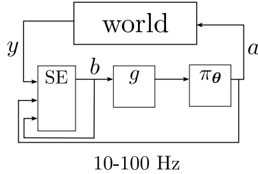
Figure 2.11: Control architecture of the apprentice robot. The control loop should run between 10-100Hz. Given an applied action, the world returns an observation which is integrated by the State Estimator (SE) to give the current belief. The belief is the compressed and given as input to the policy.
