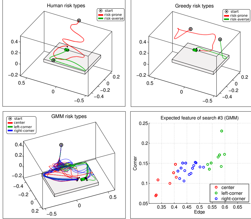
Figure 3.10: Risk prone & averse searches (red & green trajectories). Top left: Two human trajectories taken from data shown in Figure 3.9. Top right: Two Greedy trajectories. Bottom left: GMM trajectories, all starting from the same location, the colour coding is to illustrate the different policies which were encoded and emerge given the same initial conditions. Bottom right: Corresponding expected features of each trajectory, the colour coding matches the trajectories to the “GMM risk types” sub-figure. All the searches which were generated by the GMM for this initialisation produced risk-averse searches (based on the feature metric discussed previous).
