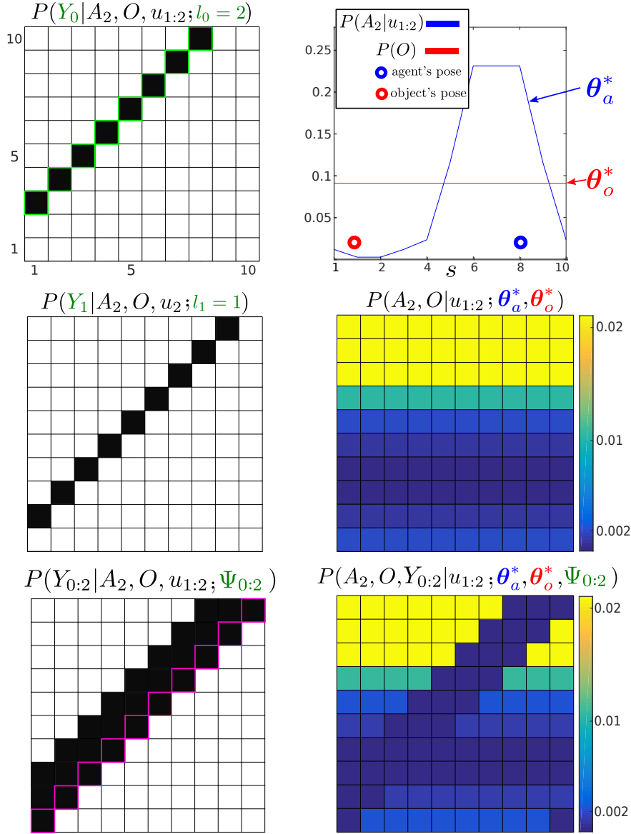
Figure 5.9: Un-normalised MLMF joint distribution, numerator of Equation 5.4.4, at time t = 2 . Three measurements (all Y = 0 ) and two actions (both u = 1 ) have been integrated into the joint distribution, for simplicity we do not consider any motion noise. Left column: The first plot illustrates the likelihood of the first measurement Y_0 . We highlight the contour in light-green to indicate that it was the first applied likelihood function (see the correspondence with Figure 5.7). The first likelihood function has been moved by the 2 actions, the second likelihood function has been moved by one action (the last one, u_2 = 1 ) and the third likelihood function has had no action applied to it yet. The last applied likelihood function is highlighted in pink and the product of all the likelihoods since t = 0 until t = 3 is depicted at the bottom of the figure which is P(Y_{0:2}|A_2, O, u_{1:2}) . Right column: the top figure illustrates the original marginal of the object P(O; \theta_o^*) , which remains unchanged, and the agent's marginal P(A_2|u_{1:2}; \theta_a^*) which has moved in accordance to the motion update function. Their product would result in the joint distribution P(A_2, O|u_{1:2}; \theta_a^*, \theta_o^*) illustrated in the middle figure if evaluated at each state (i, j) . The bottom figure is the result of multiplying P(A_2, O|u_{1:2}; \theta_a^*, \theta_o^*) with P(Y_{0:2}|A_2, O, u_{1:2}; \Psi_{0:2}) giving the filtered joint distribution, Equation 5.4.4.
