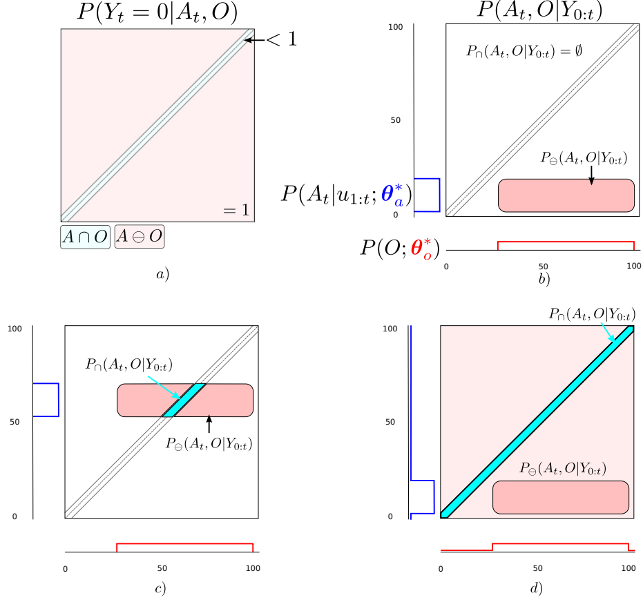
Figure 5.10: a) Likelihood P(Y_t = 0|A_t, O) , the blue area depicts the regions in which the likelihood is < 1 and the red area is where the likelihood is = 1 . If the probability mass of the joint distribution is in the blue region, then the parameters of the random variables in these areas are dependent, A \cap O . Otherwise they are independent, A \ominus O . b) The agent and object marginals are not overlapping and are thus completely independent. The joint distribution, P(A_t, O|Y_{0:t}) the black rectangle, is not intersecting with the measurement function. As a result P_{\cap}(A_t, O|Y_{0:t}) is empty. c) The marginals overlap resulting in the measurement likelihood intersecting with the joint distribution. The joint distribution is composed of the blue and red areas, Equation 5.4.10. The probability mass at the intersection is removed and re-normalised to other regions which is the result of applying Bayes integration. d) The marginals of A and O are completely overlapping, however only a small fraction of the probability mass in the joint distribution is within the measurement function's tube.
