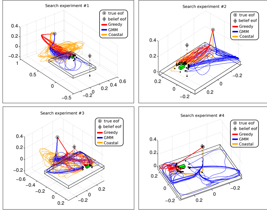
Figure 3.13: Four search initializations, from top left to bottom right we refer to them as #1-4. The circle indicates the true starting point of the end-effector (eof), whilst the triangle is the initial believed location of the eof. The initialisation in #1 was chosen such that the true and believed eof locations were at opposite sides of the table. This setting was selected to highlight the draw back in methods which do not take into account uncertainty. The second initialisation #2, reflects the situation where once again there is a large distance between true and believed location of the eof. However this time both are above the table. The starting points in #3 are a variant on #1 with the difference being that the believed eof position is above the table whilst the true eof location is not. The last experiment #4 was a setup which would be favourable to algorithms that are inclined to be greedy. Both true and believed eof locations are close to one another.
