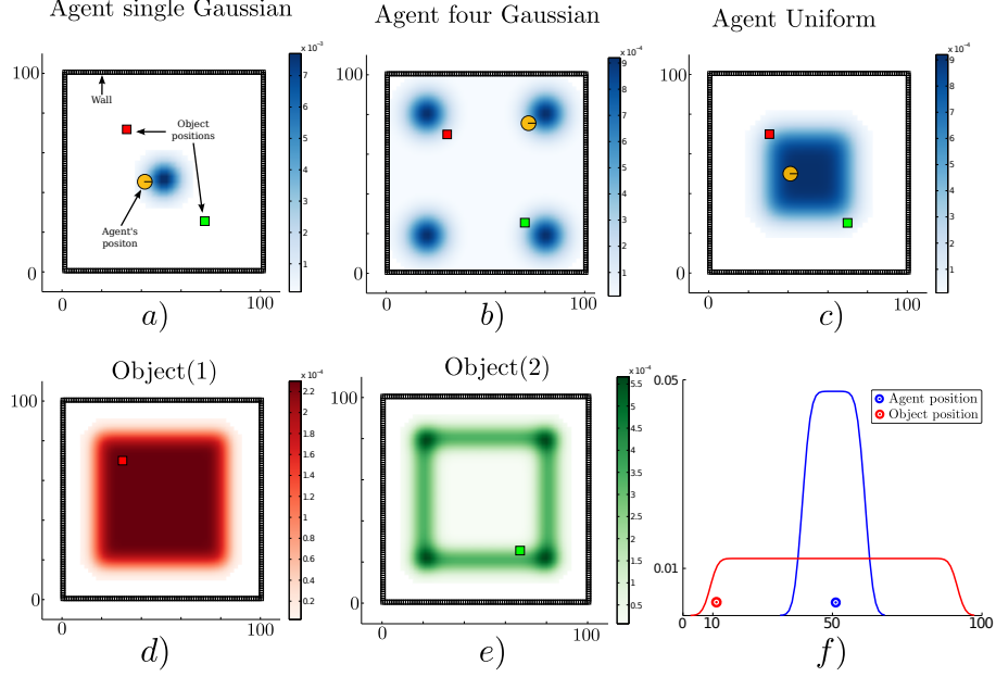
Figure 5.17: Agent's prior beliefs. Two types of environment, the first is a 2D world where the agent lives in a square surrounded by a wall whilst the second is a 1D world. In the 2D figures the agent is illustrated by a circle with a bar to indicate its heading. The true location of the objects are represented by colour coded squares. Top row three different initialisations of the agent's location. Bottom row d) the agent's prior beliefs with respect to the location of the first object and e) belief of the second object's location. bottom row f) 1D world with one object.
