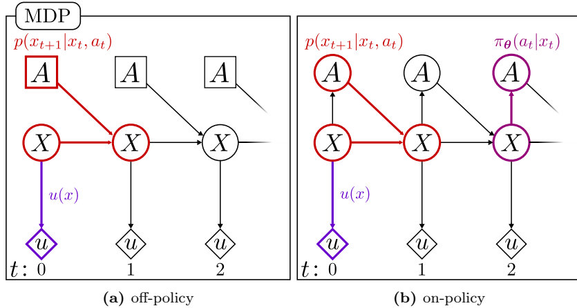
Figure 2.3: Dynamical Bayesian Network of a Markov Decision Process; it encodes the temporal relation between the random variables (circles), utilities (diamond) and decisions (squares). The arrows specify conditional distributions. In (a) the decision nodes are not considered random variables whilst in (b) they are. From these two DBN we can read off two conditional distributions, the state transition distribution (in red) and the action distribution (in purple).
