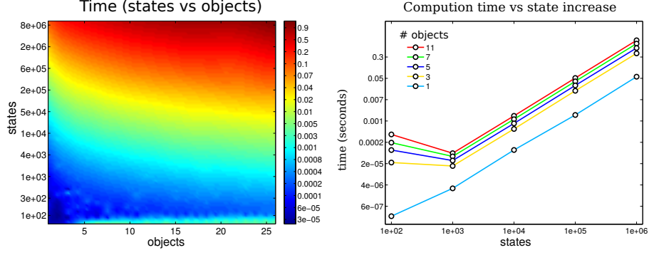
Figure 5.15: Time complexity: left: mean time taken for a loop update (motion and measurement) as a function of the number of states in a marginal and the number of objects present. right: time taken for a loop update with respect to the number of states in the marginal. The colour coded lines are associated with the number of objects present. The computational cost is plotted on a log scale. As the number of states increases exponentially the computational cost matches it.
