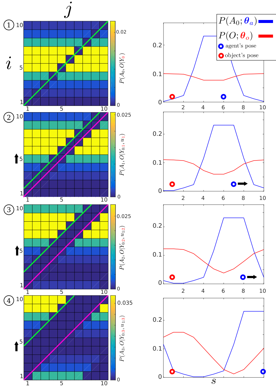
Figure 5.7: Histogram-SLAM, 4 time steps. 1 Application of likelihood P(Y_0 = 0|A_0, O) and the agent remains stationary, u_1 = 0 , all states along the green line become zero. 2 The agent moves to the right u_1 = 1 , the motion P(A_1|A_0, u_1) , and likelihood models are applied consecutively. The right motion results in a shift (black arrow on the left) in the joint probability distribution towards the state i = 10 . All parameters on the pink line are zero. 3 Same as two. 4 The original result of the likelihood function, green line, has moved by the same amount as the agent's displacement. At each time step a new likelihood function (pink line) is applied to the joint distribution.
