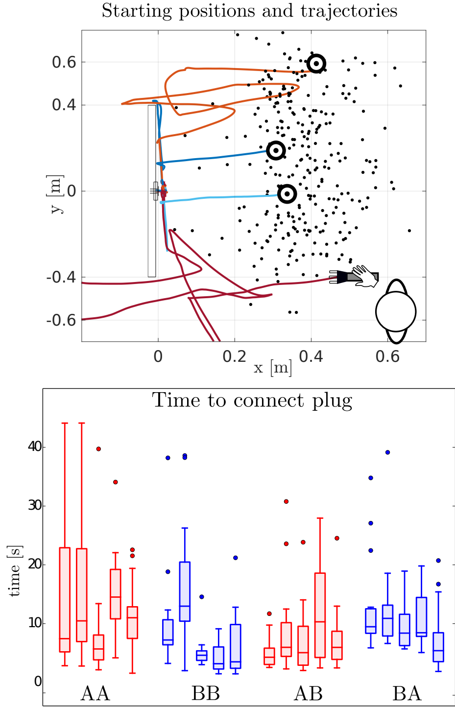
Figure 4.6: Top: Black points represent the starting position of the end-effector for all the demonstrations. Four trajectories are illustrated. Bottom: Time taken for the teachers to accomplish the PiH once the socket is localised. Group A and B are depicted in red and blue. The second later indicates which socket is used, see Figure 4.5.
