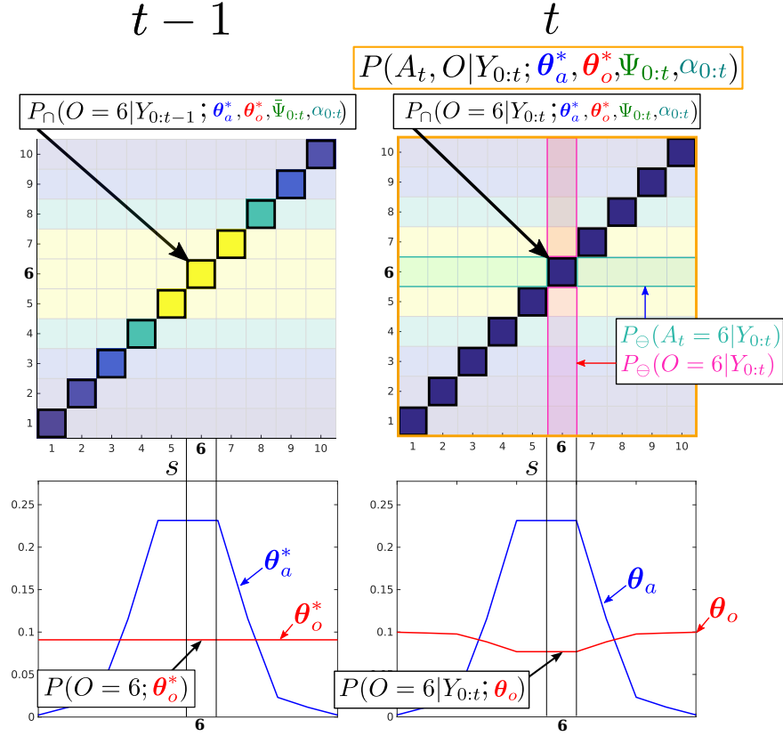
Figure 5.11: Filtered marginals. Illustration of the agent and object marginal update, Equation 5.4.13. The joint distribution parameters which are independent A \ominus O are pale and the dependent areas A \cap O , where P(Y_t < 1|A_t, O) , are bright. MLMF only evaluates the joint distribution in dependent states. For each state s of the marginals 1, \dots, 10 the difference of the marginals inside the dependent area, before and after the measurement likelihood is applied, is evaluated and removed from the marginals P(A_t|Y_{0:t-1}, u_{1:t}; \theta_a) , P(O|Y_{0:t-1}; \theta_o) leading to P(A_t|Y_{0:t}, u_{1:t}; \theta_a) , P(O|Y_{0:t}; \theta_o) (we did not show u_{1:t} in the figure for ease of notation). Bottom-left: joint marginals P(A_t|u_{1:t}; \theta_a^*) and P(O; \theta_o^*) remain unchanged by measurements.
