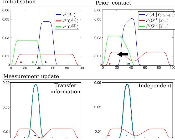
Figure 5.14: Transfer of information (marginals) Top left: Initial beliefs of the agent and object’s location. The agent moves to the left until it senses object O^{(2)} . Top right: Marginals prior the agent entering in contact with the green object, see Figure 5.13 ( Top ) for an illustrate of the joint distributions. The black arrow indicates the heading of the agent. Bottom left: resulting marginals after setting the agent marginals of each joint distribution equal A_t^{(1)} = A_t^{(2)} according to Algorithm 4. The object marginal P(O^{(2)}|Y_{0:t}) is recomputed. Bottom right: resulting marginals in which the objects have no influence on one another. Note that a transfer of information has caused a change in the marginal O^{(1)} .
