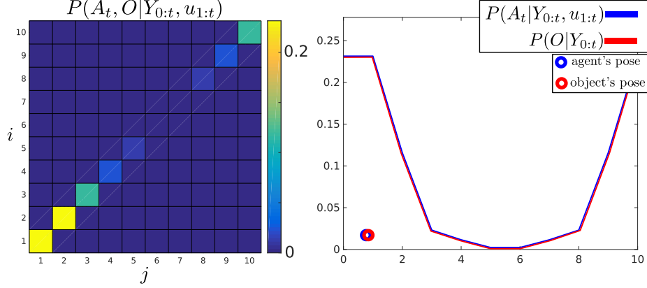
Figure 5.8: Histogram-SLAM contact. The agent has entered in contact with the object (measurement Y_t = 1 ) and the likelihood function P(Y_t = 1|A_t, O) is applied to the joint distribution. Only parameters on the line i = j will remain unchanged and parameters for which i \neq j will be set to zero.
