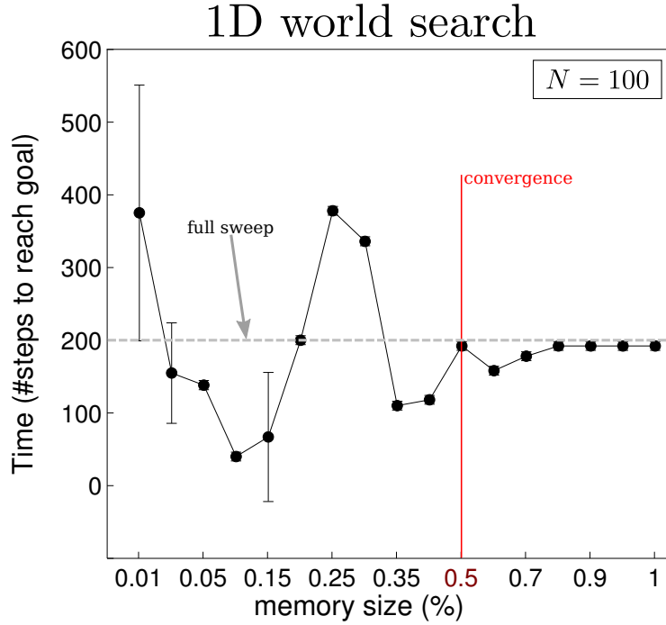
Figure 5.18: Memory size vs time to find object in 1D Results of the effect of the memory size on the decision process for the 1D search illustrated in Figure 5.17 f). The memory size is reported as the percentage of total number of states present in the marginal space. At 100% the size of the memory is equal to that of the state space, N = 100 in this case. A total sweep of the entire state space would result in a total of 200 steps, the dotted grey line in the above figure. When no restrictions are placed on the memory size the policy following the greedy approach takes around 180 steps. This result converges when the number of parameters |\Psi_{0:t}| of the memory likelihood function is greater than 50% of the original state space.
