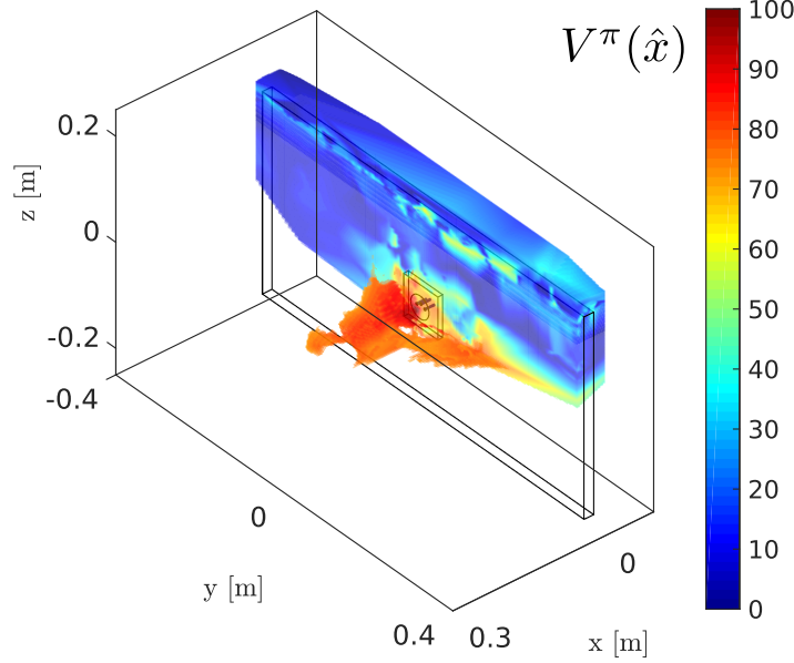
Figure 4.18: Value function learned from the 15 demonstrations of teacher #5. The value of the most likely state is plotted.
