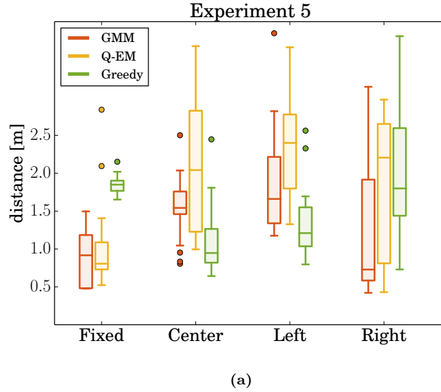
Figure 4.22: Distance taken to reach the socket's edge. For the Fixed setup (see Figure 4.21) for the initial condition), both the Q-EM and GMM significantly outperform the Greedy.
