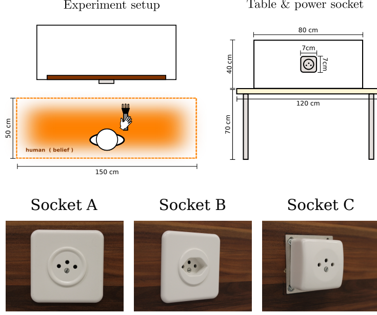
Figure 4.2: The experimental setup. Top-left: A participant (human teacher) is blindfolded and placed within the orange rectangular area always facing the wall. Top-right: Dimensions of the the wall and socket. Bottom: Three different power sockets, only socket A and B are used for data collection, socket C is purely used for evaluating the generalisation of the learned policy.
