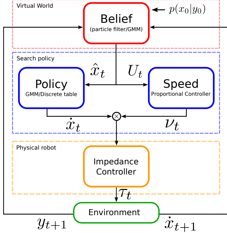
Figure 3.7: Overview of the decision loop. At the top a strategy is chosen given an initial belief p(x_0|y_0) of the location of the end-effector (initially through sampling the conditional). A speed is applied to the given direction based on the believed distance to the goal. This velocity is passed onwards to a low level impedance controller which sends out the required torques. The resulting sensation, encoded through the Multinomial distribution over the environment features, and actual displacement are sent back to update the belief.
