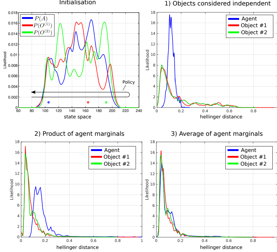
Figure 5.16: Comparison of scalable-MLMF and the histogram filter A deterministic sweep policy was carried out for 100 different initialisations of the agent and object beliefs. Top left: One particular Initialisation of the agent and object random variables. The true position of the agent and objects were sampled at random. The black arrow indicates the general policy which was followed for each of the 100 sweeps. These were performed for 1) scalable-MLMF with objects considered to be independent at all times (no Algorithm 4). 2) Agent marginal P(A_t|Y_{0:t}, u_{1:t}) is the product of marginals P(A_t^{(i)}|Y_{0:t}^{(i)}, u_{1:t}) , Equation 5.4.17. 3) marginal P(A_t|Y_{0:t}, u_{1:t}) is taken to be the average of all marginals P(A_t^{(i)}|Y_{0:t}^{(i)}, u_{1:t}) , Equation 5.4.18. For each of these three experiment we report the kernel density estimation over the Hellinger distances taken at every time step between ground truth (from histogram filter) and scalable-MLMF.
