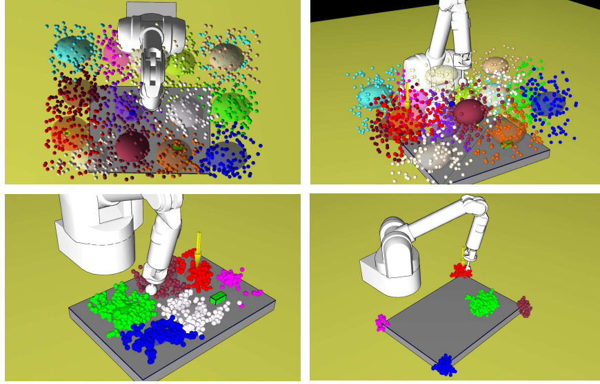
Figure 3.5: Representation of the estimated density function. Top Left and Right: Initial starting point, all Gaussian functions are uniformly distributed with uniform priors. The red cluster always has the highest likelihood which is taken to be the believed location of the robot’s/human’s end-effector. Bottom Left: Contact with the table has been established, the robot location differs from his belief. Bottom Right: Contact has been made with a corner, the clusters reflect that the robot could be at any corner (note that weights are not depicted, only cluster assignment).
