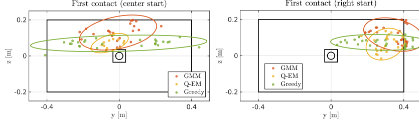
Figure 4.14: First contact with the wall, during experiment 1. (a) Contact distribution for initial condition “Center” . (b) Contact distribution for initial condition was “Right”. The ellipses correspond to two standard deviations of a fitted Gaussian function.
