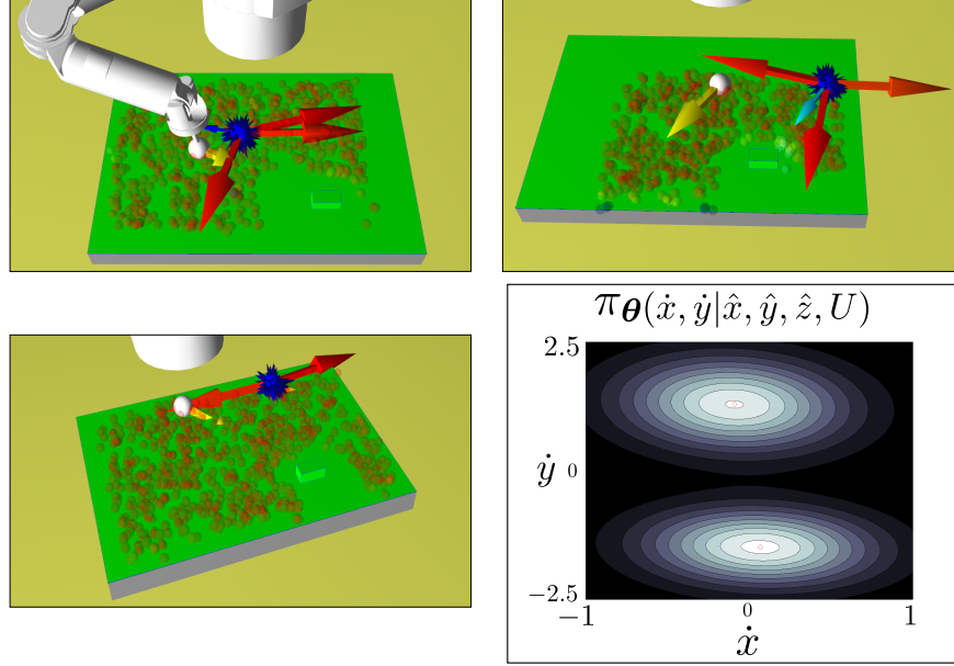
Figure 3.11: Illustration of three different types of modes present during the execution of the task where the robot is being controlled by the learned GMM model. The white ball represents the actual position of the robot's end-effector. The blue ball represents the believed position of the robot's end-effector and the robot is acting according to it. The blue ball arrows represent modes. Colours encode the mode's weights given by the priors \pi_k after conditioning ( but not re-weighted as previously described). The spectrum ranges from red (high weight) to blue (low weight). Top left: Three modes are present, but two agree with each other. Top right: Three modes are again present indicating appropriate ways to reduce the uncertainty. Lower left: Two modes are in opposing directions. No flipping behaviour between modes occurs since preference is given to the modes pointing in the same direction as the robot's current trajectory. Lower right: GMM modes when conditioned on the state represented in the lower left figure. The two modes represent the possible directions (un-normalised).
